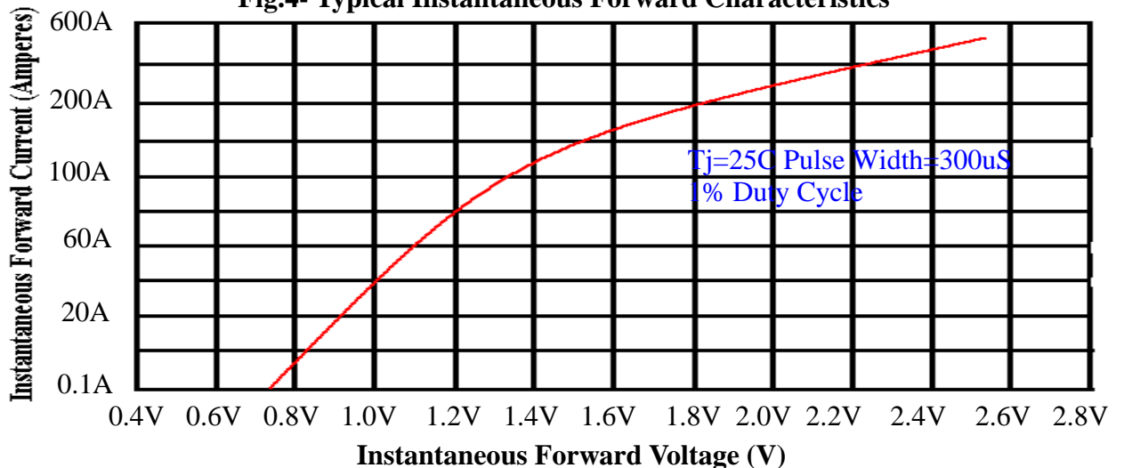
Fig.4- Typical Instantaneous Forward Characteristics
