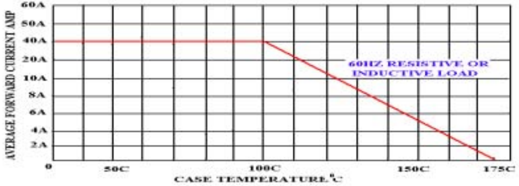
FIG.1 –FORWARD CURRENT DERATING CURVE
