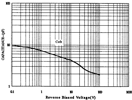
CAPACITANCE VS REVERSE-BIASED VOLTAGE
