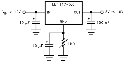
Adjusting Output of Fixed Regulators
