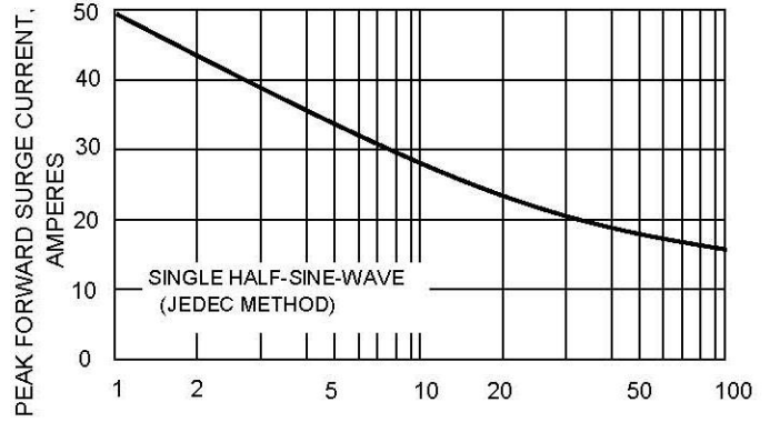
FIG.2-MXIMUM NON-REPETITIVE SURGE CURRENT
