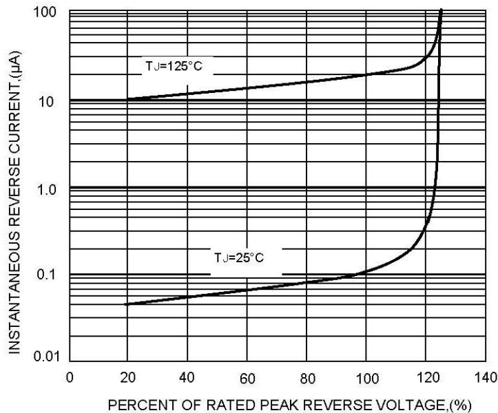
FIG.5-TYPICAL REVERSE CHARACTERISTICS
