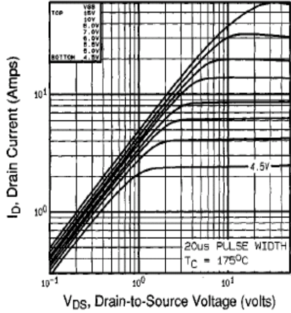
Fig 2. Typical Output Characteristics, T_C=175^\circ\text{C}
