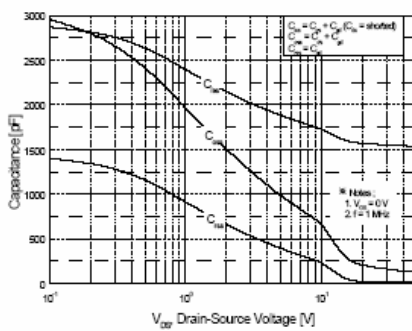
Figure 5. Capacitance Characteristics
