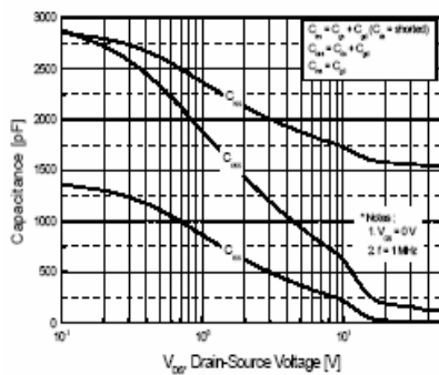
Figure 5. Capacitance Characteristics
