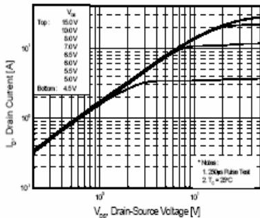
Figure 1. On-Region Characteristics
