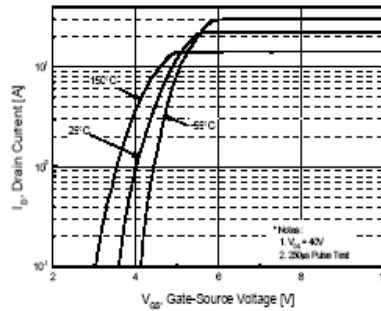
Figure 2. Transfer Characteristics
