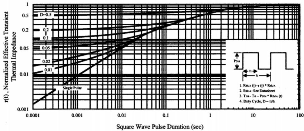
Figure 10. Normalized Thermal Transient Impedance Curve
