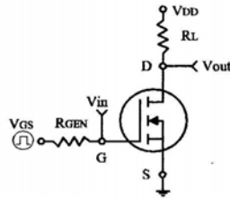
Figure 9. Switching Test Circuit and Switching Waveforms
