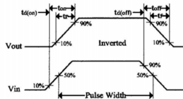
Figure 9. Switching Test Circuit and Switching Waveforms
