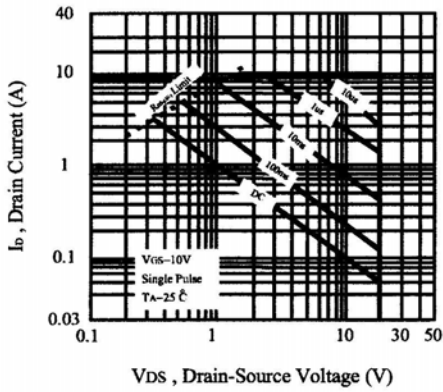
Figure 7. Maximum Safe Operating Area
